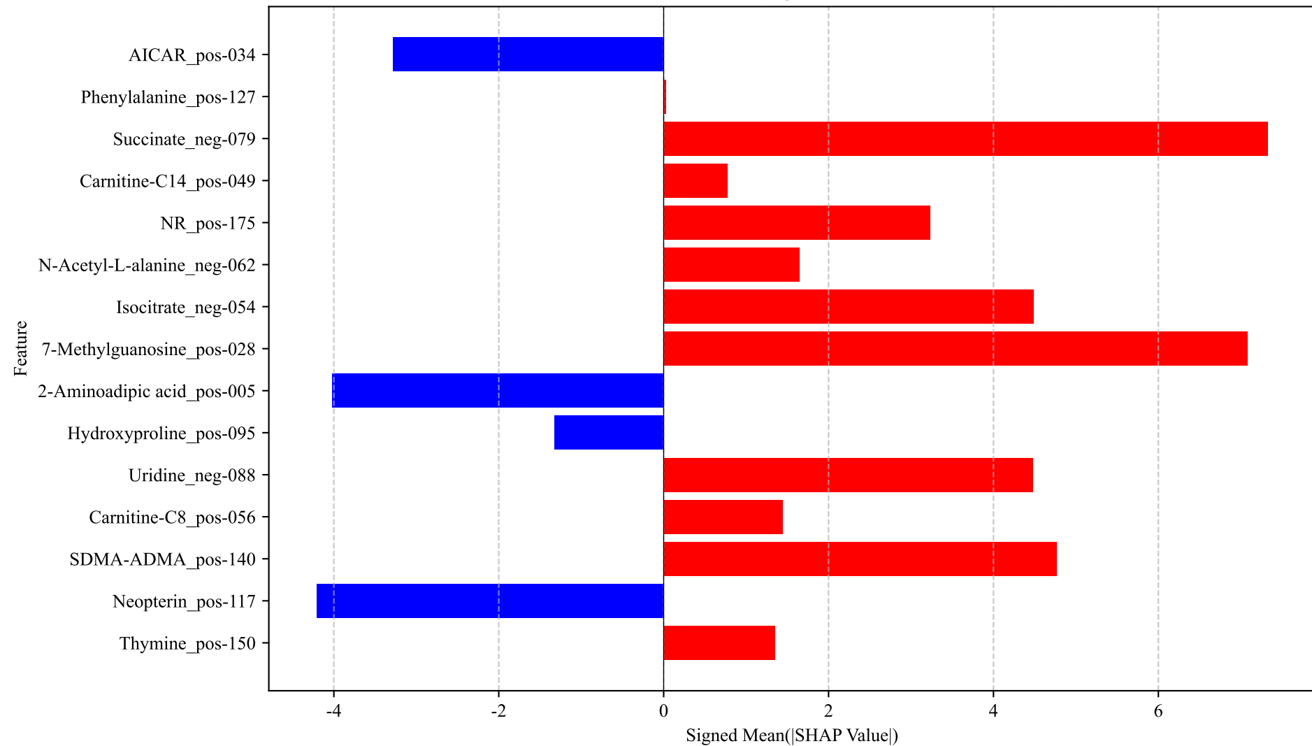
SHAP Values for Test Set (Signed Mean of Absolute Values)
